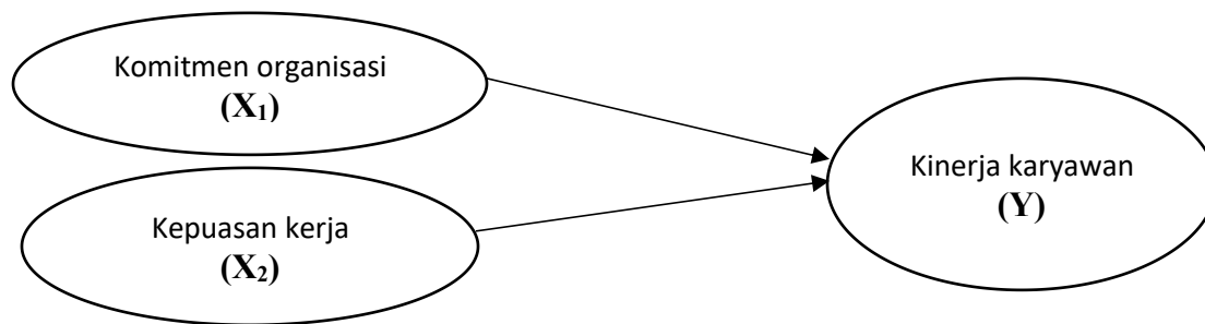
Gambar 1 Model Penelitian
